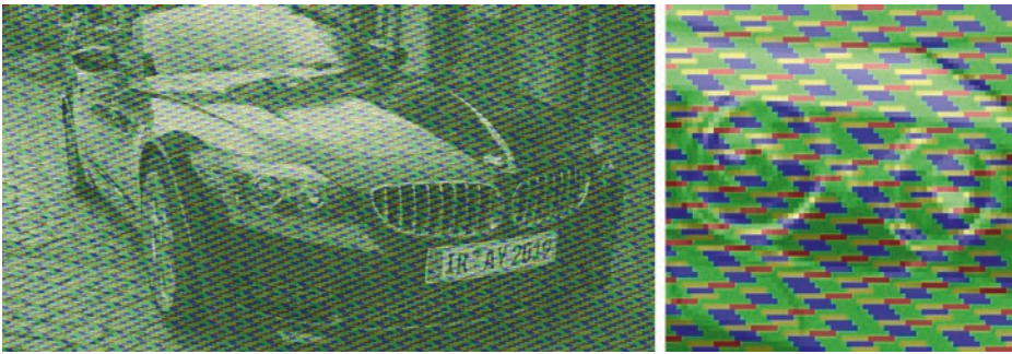
Figure 10-2. Adaptive tiling for four processing units with relative weights of 10% (red), 15% (yellow), 25% (blue), and 50% (green). Note how the headlight pixels are distributed among processing units.
