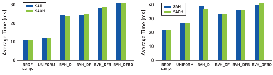
Figure 18-6. Comparisons in Bistro (view 1) (left) and PBG-R (right) of rendering times in milliseconds per frame using the different traversal methods, compared to sampling the BRDF to get the light sample direction. All methods use 4 samples per pixel, and BVH-based methods use 16 bins along all three axes.
